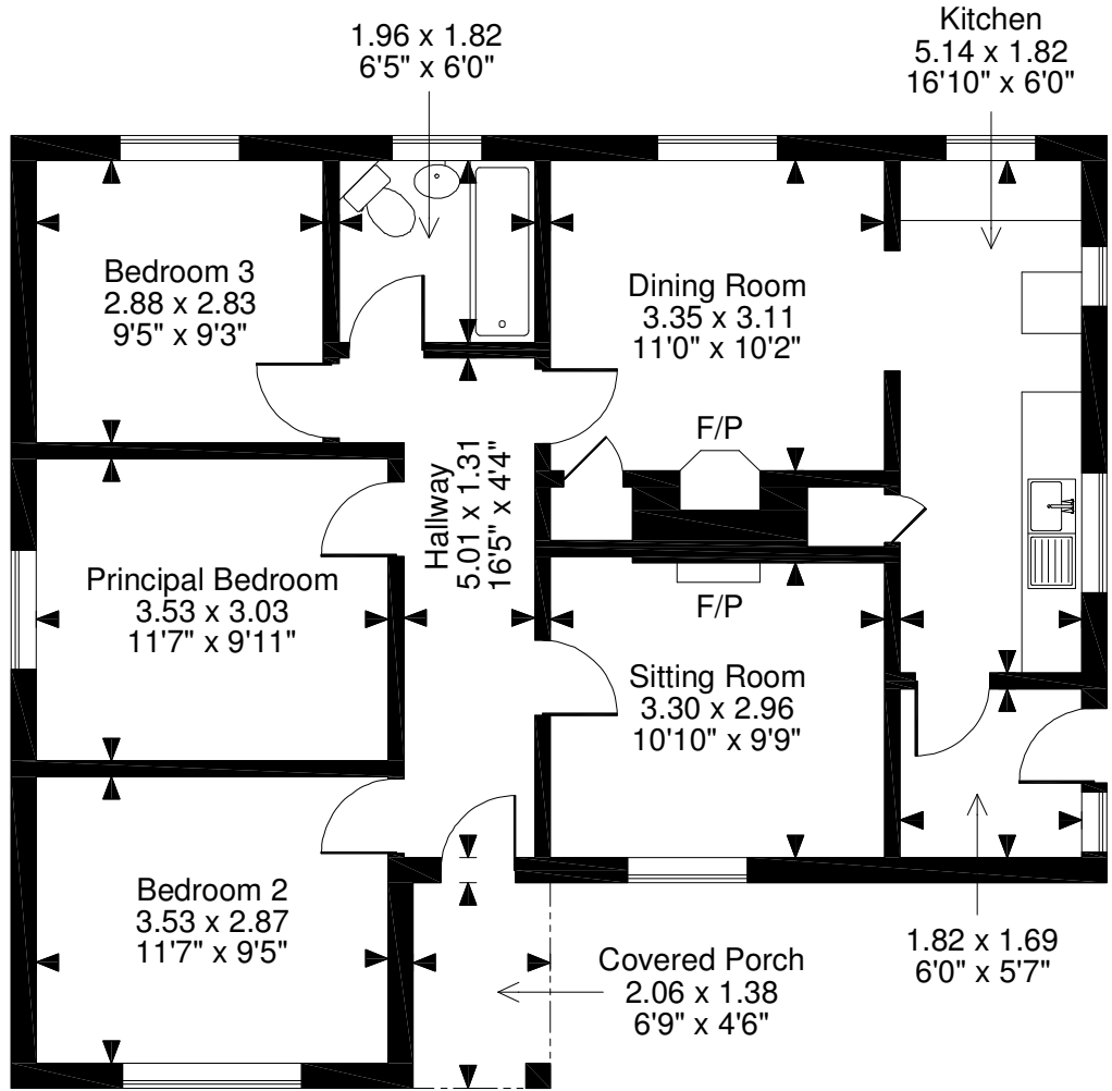
Ground Floor
